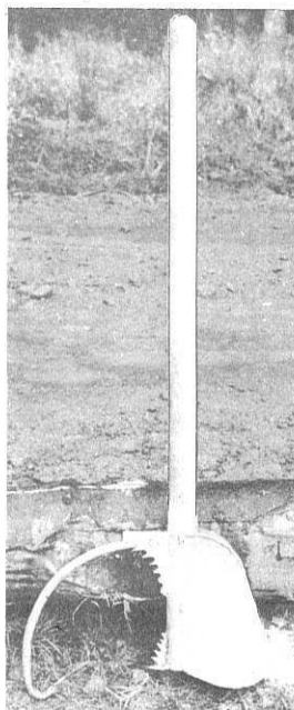
7. Log Jack
