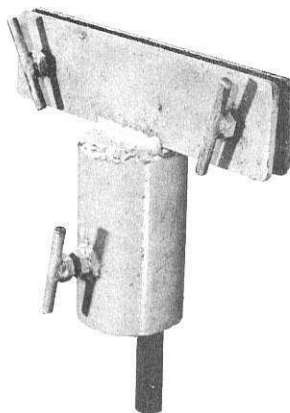
7. Pruning Saw Vice
